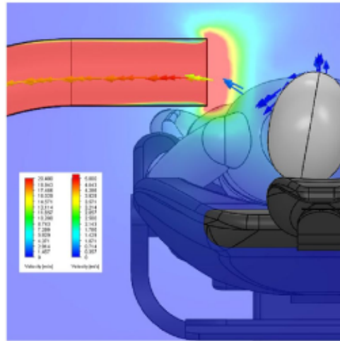
5" diameter vacuum hose on side without the AirGuard™ XP
