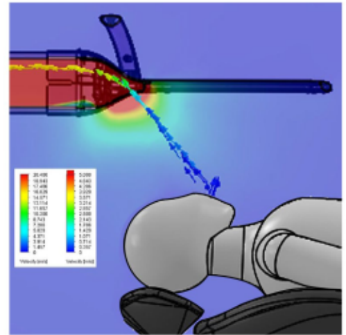
5" diameter vacuum hose overhead with the AirGuard™ XP
