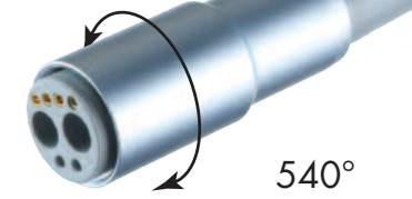
Silicone hose with connector for use with DEFINITIVE®LED or Bien-Air MC3 IK/LED motors
