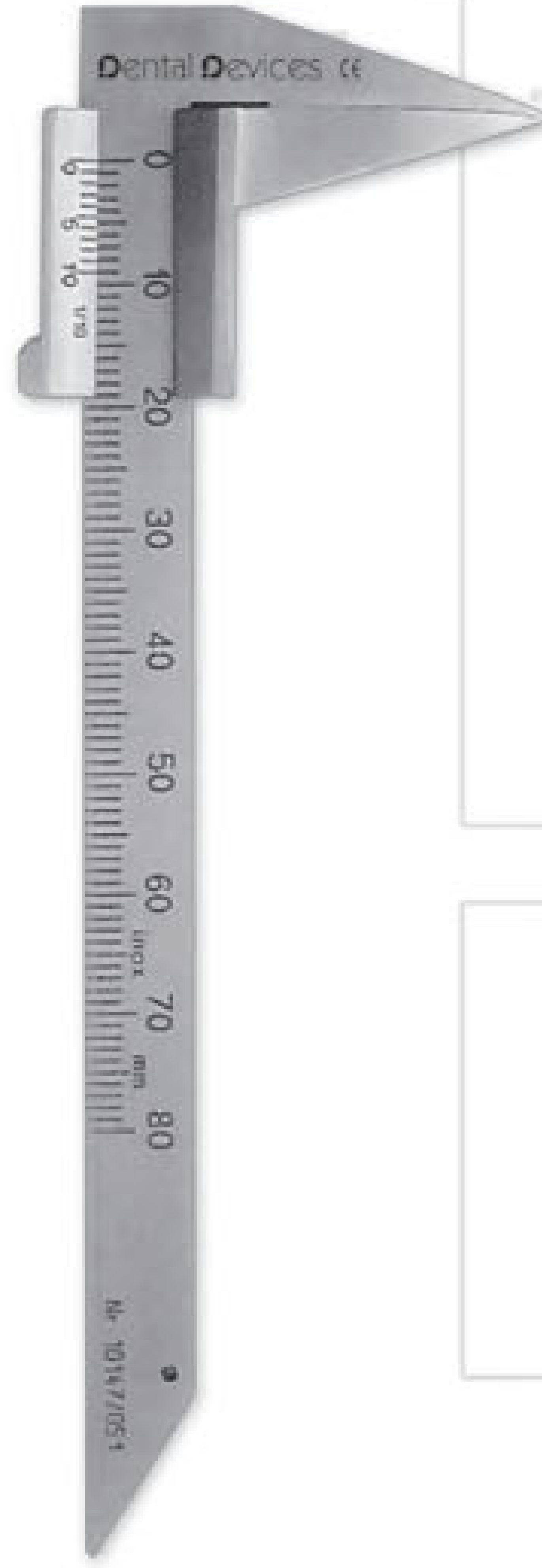
DD-137 Dental Caliper Single Point Curved 13cm
